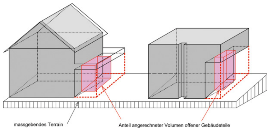
Figur 7.3 Baumassenziffer
